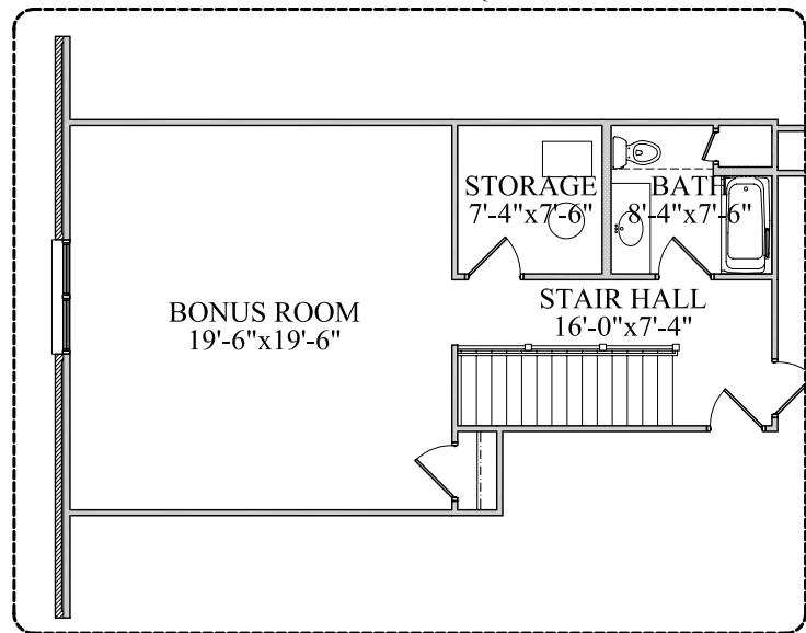
OPTIONAL BONUS ROOM *ADDS 454 SQUARE FEET*
