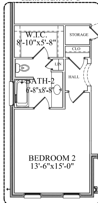
OPTIONAL BEDROOM LAYOUT "B"
